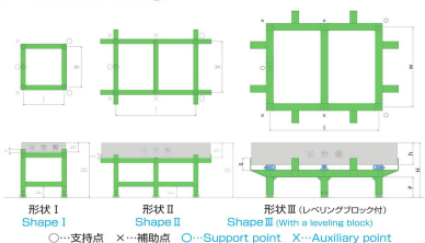
■寸法図 Dimensional drawings
